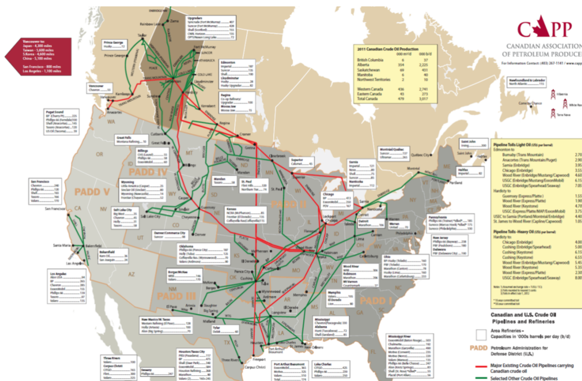
Figure 1-2: Existing North American Crude Oil Pipeline Network
